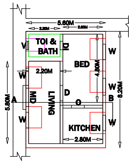
GROUND FLOOR PLAN SCLAE 1:100
