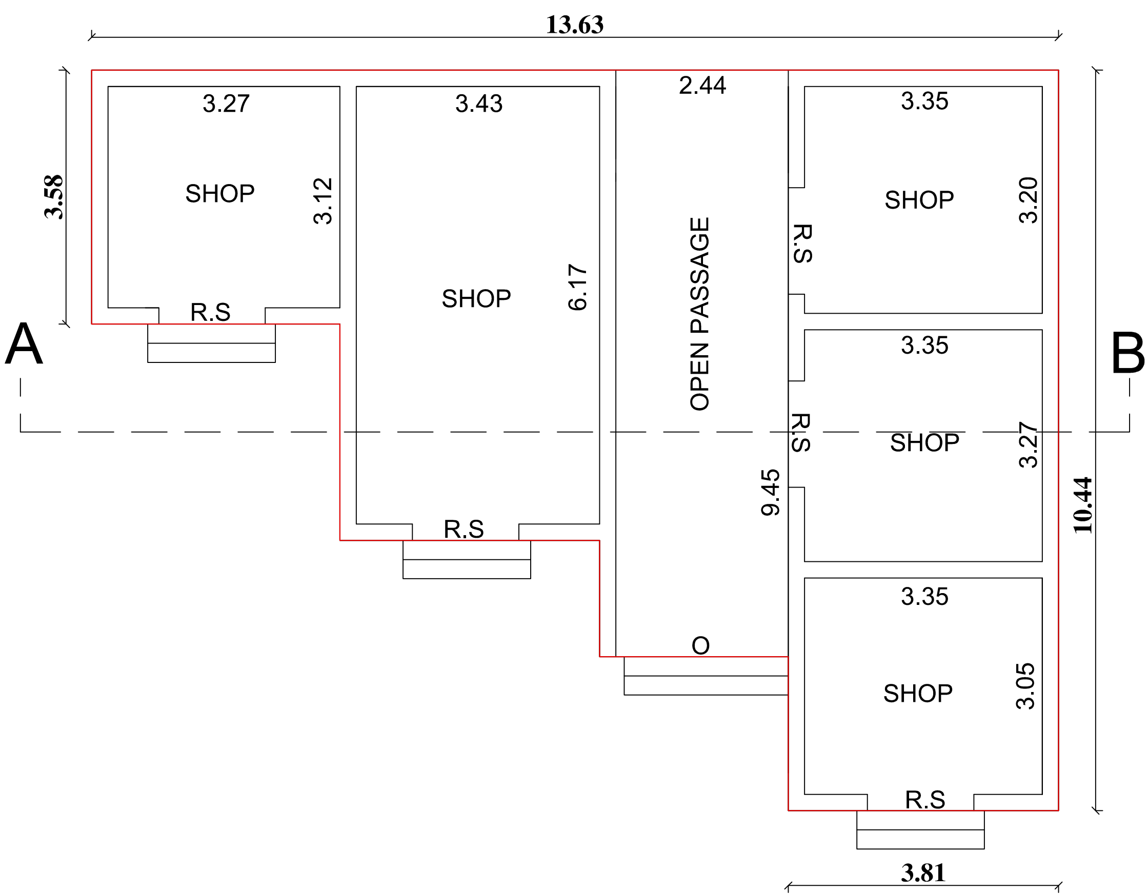
PLAN
