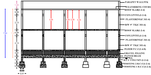
SECTION AA1
