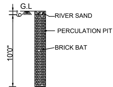
PERCULATION PIT
