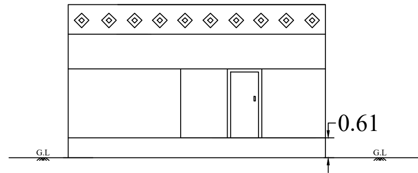
FRONT ELEVATION
