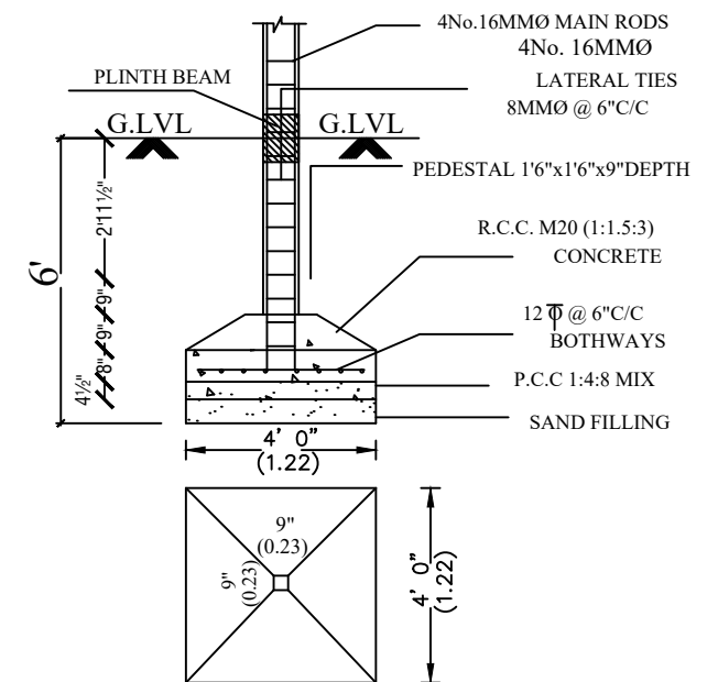
FOUNDATION DETAIL
