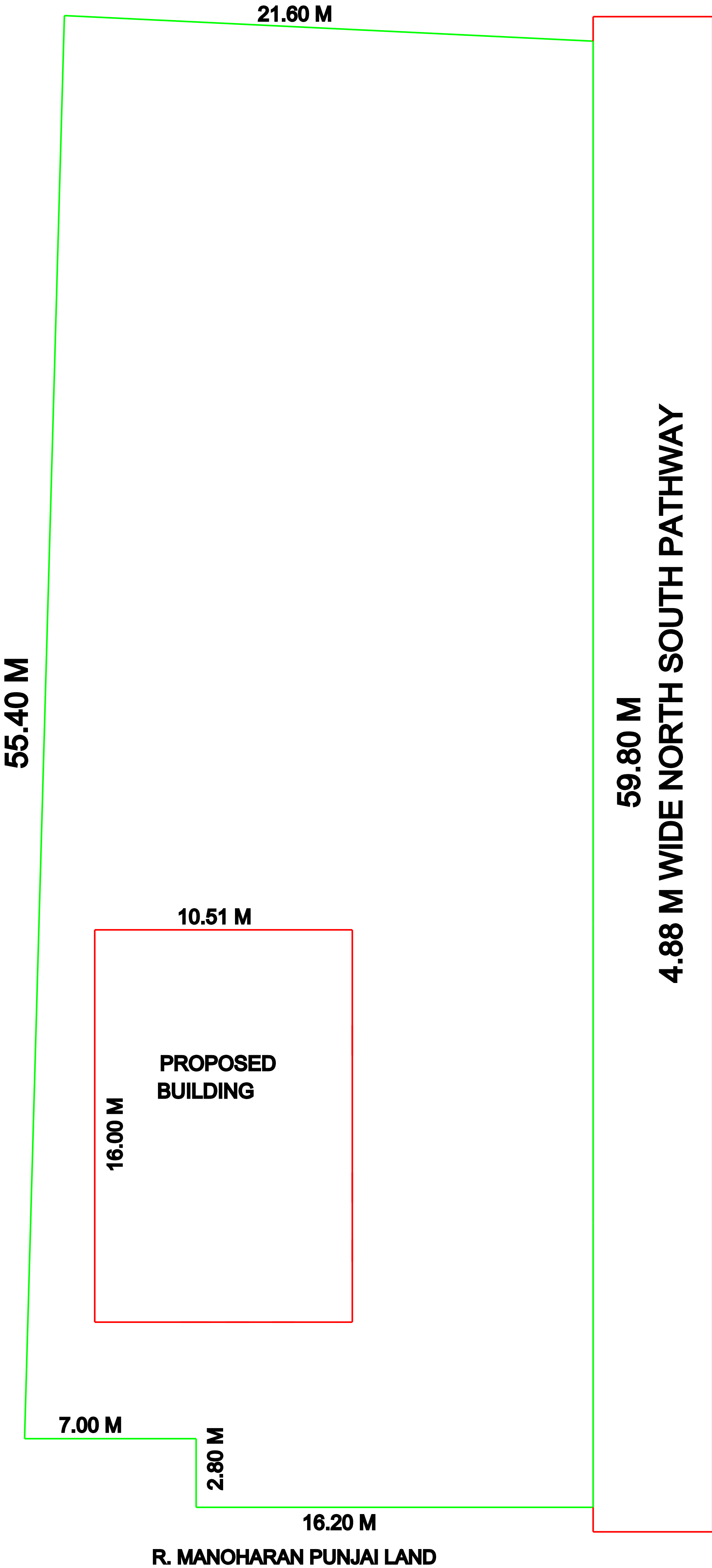
SITE PLAN
