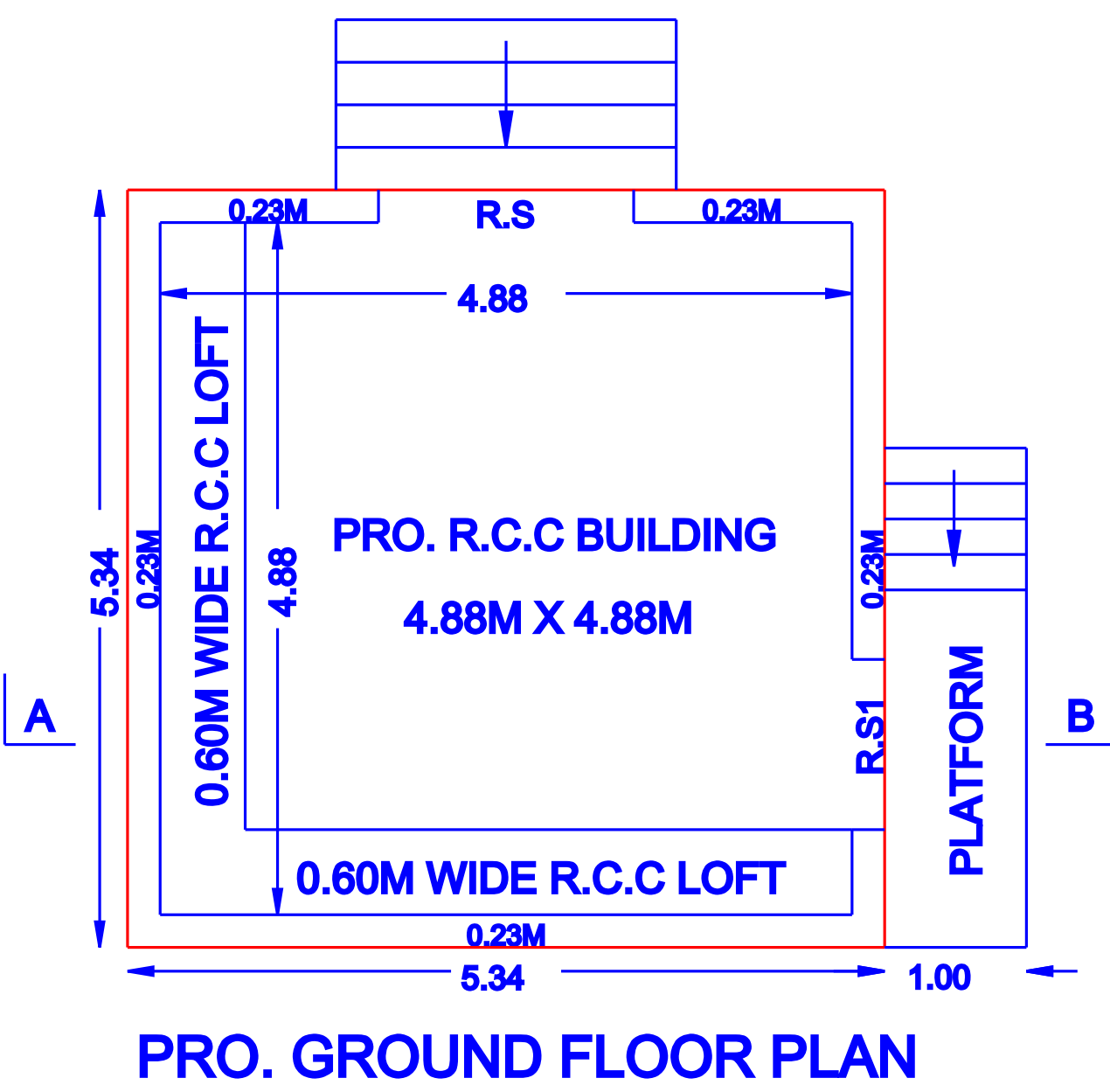
PRO. R.C.C BUILDING
