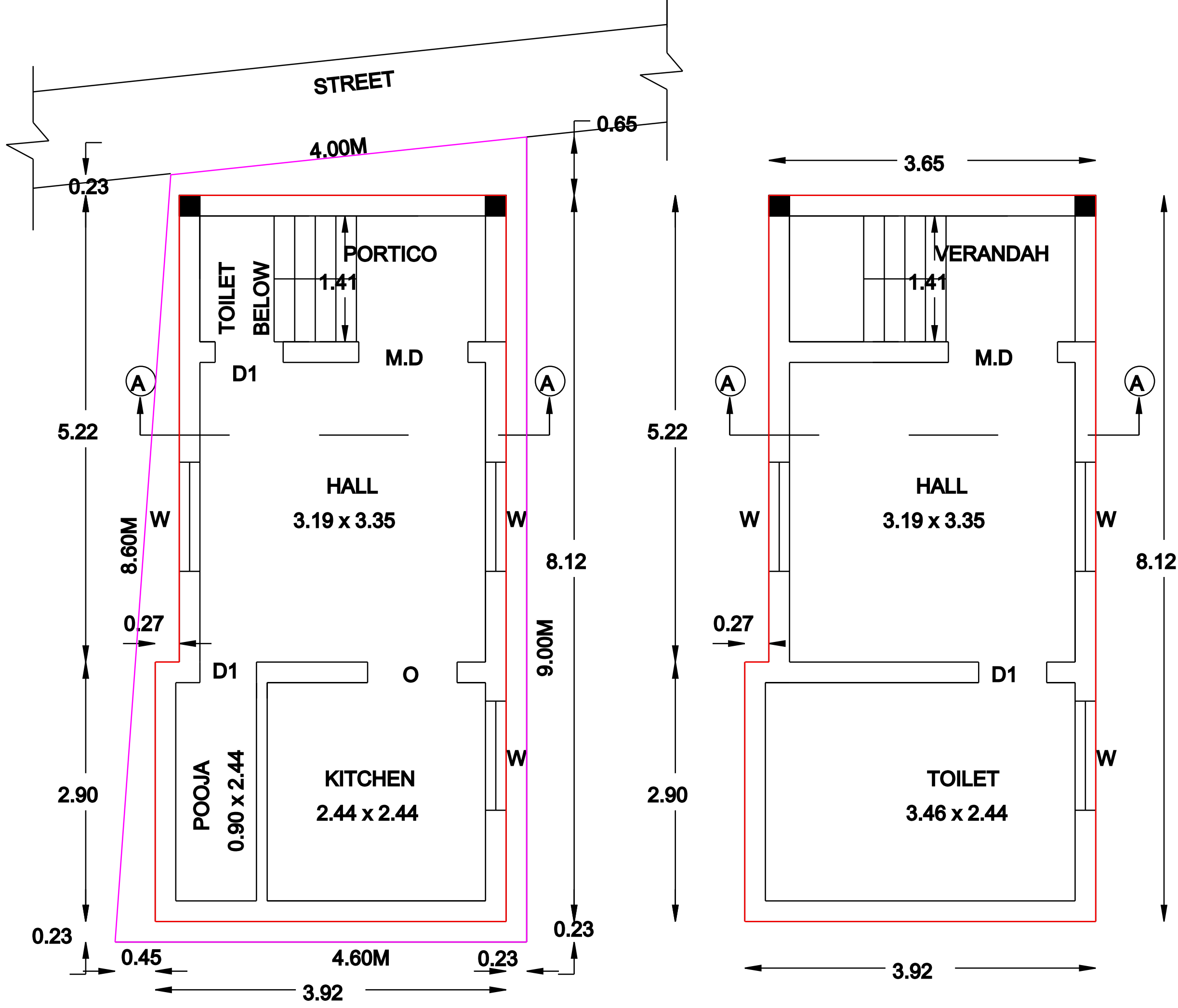
FLOOR PLAN
