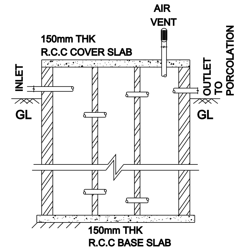
SECTION Z-Z
