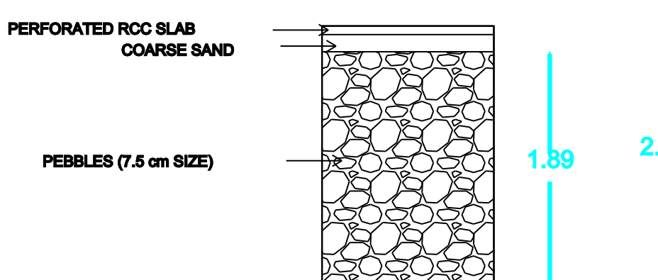
RAIN WATER HARVESTING
