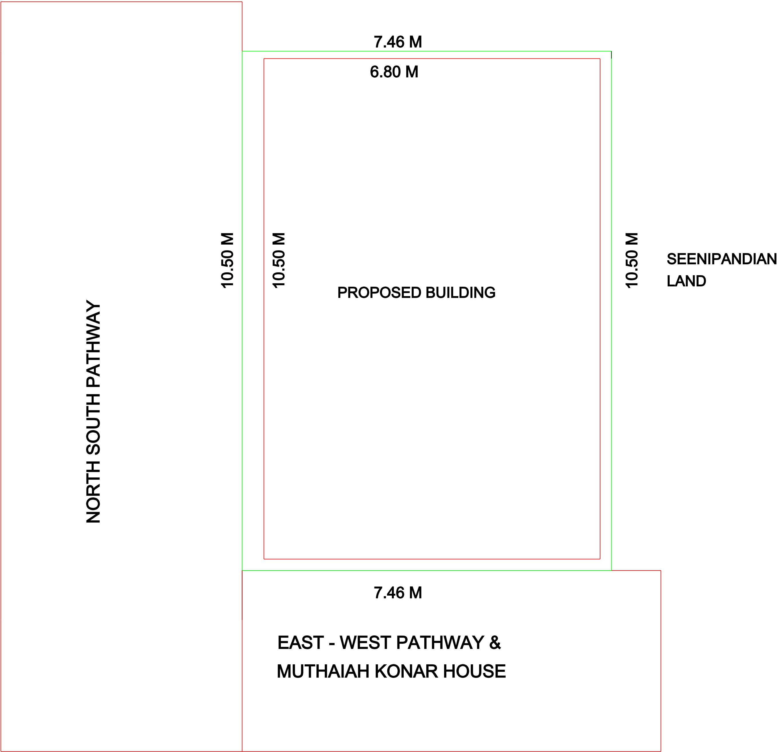
SITE PLAN
