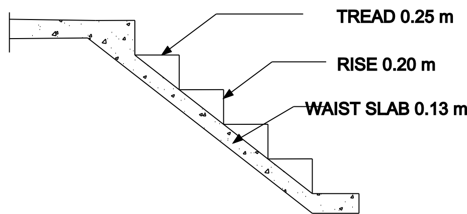
STAIR DETAILS
