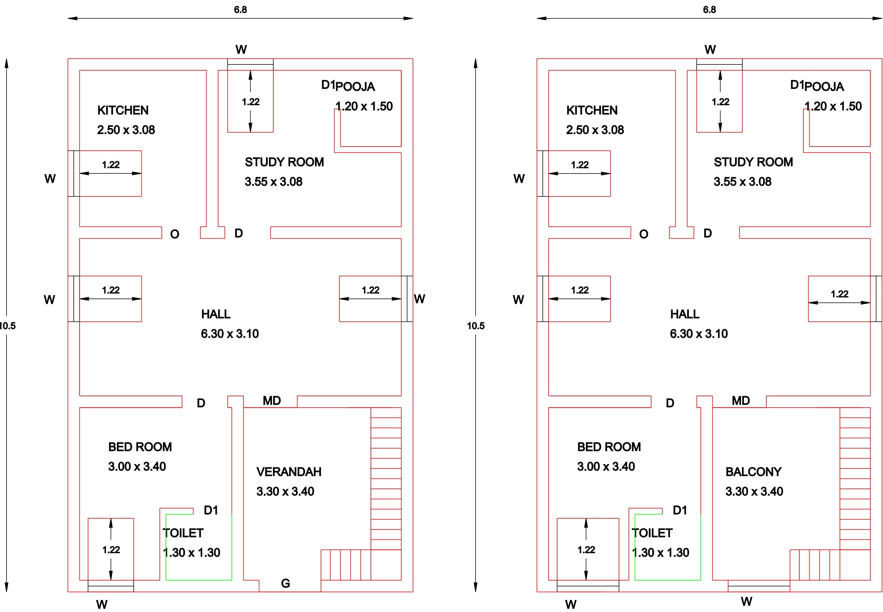
PROPOSED FIRST FLOOR
