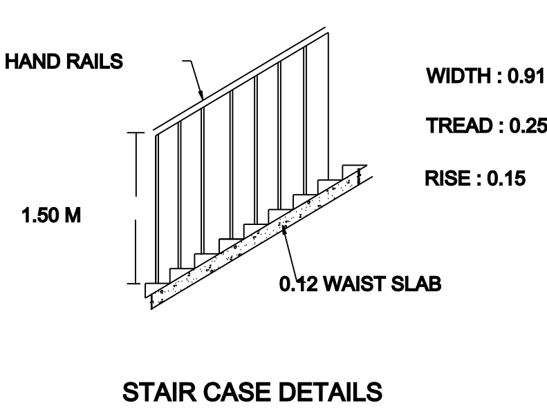
STAIR CASE DETAILS
