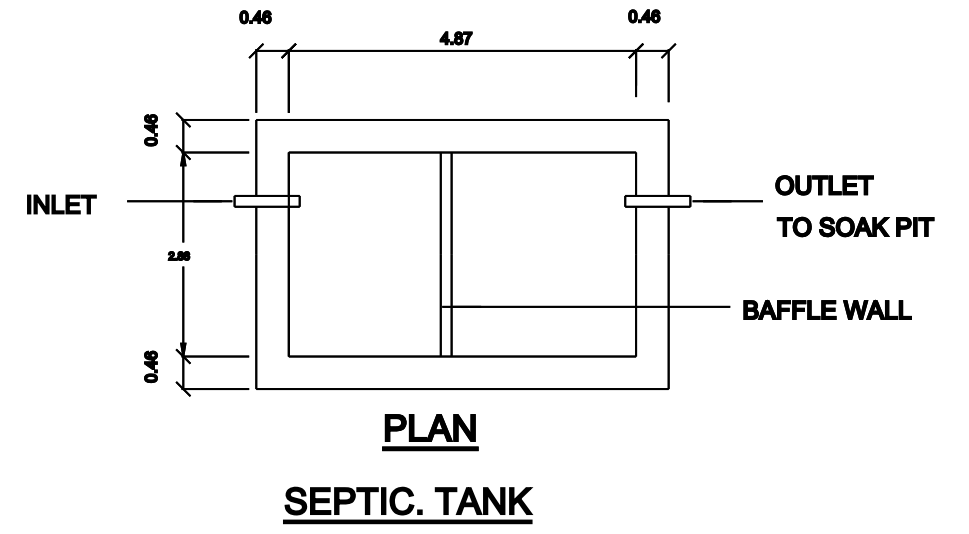
SEPTIC TANK
