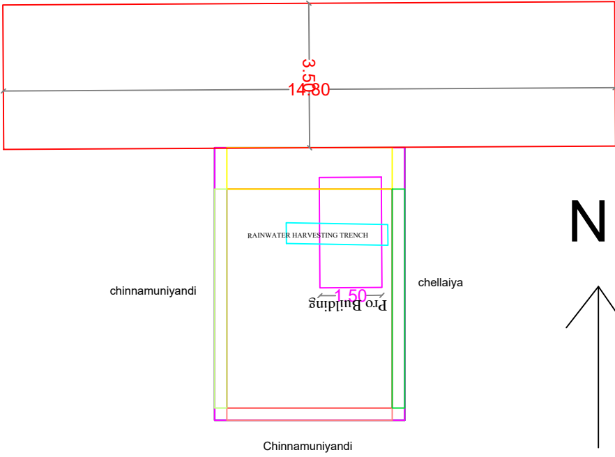
SITE PLAN
