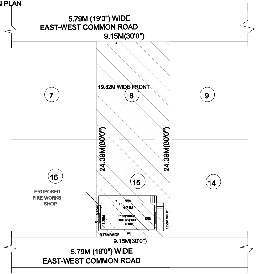
LOCATION PLAN
