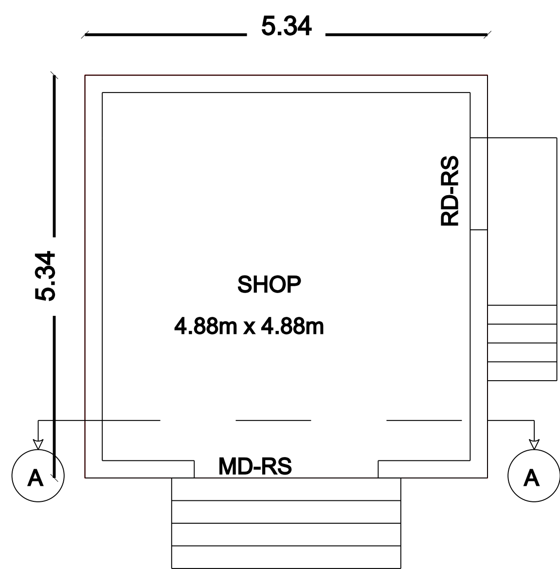
FLOOR PLAN
