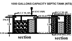
LEACH WELL DETAIL
