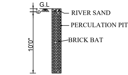
PERCOLATION PIT
