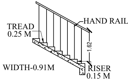
STAIRCASE DETAILS
