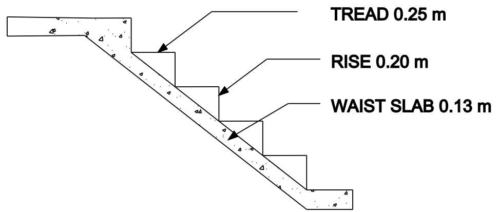
STAIR DETAILS
