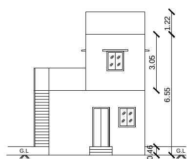
EAST SIDE ELEVATION
