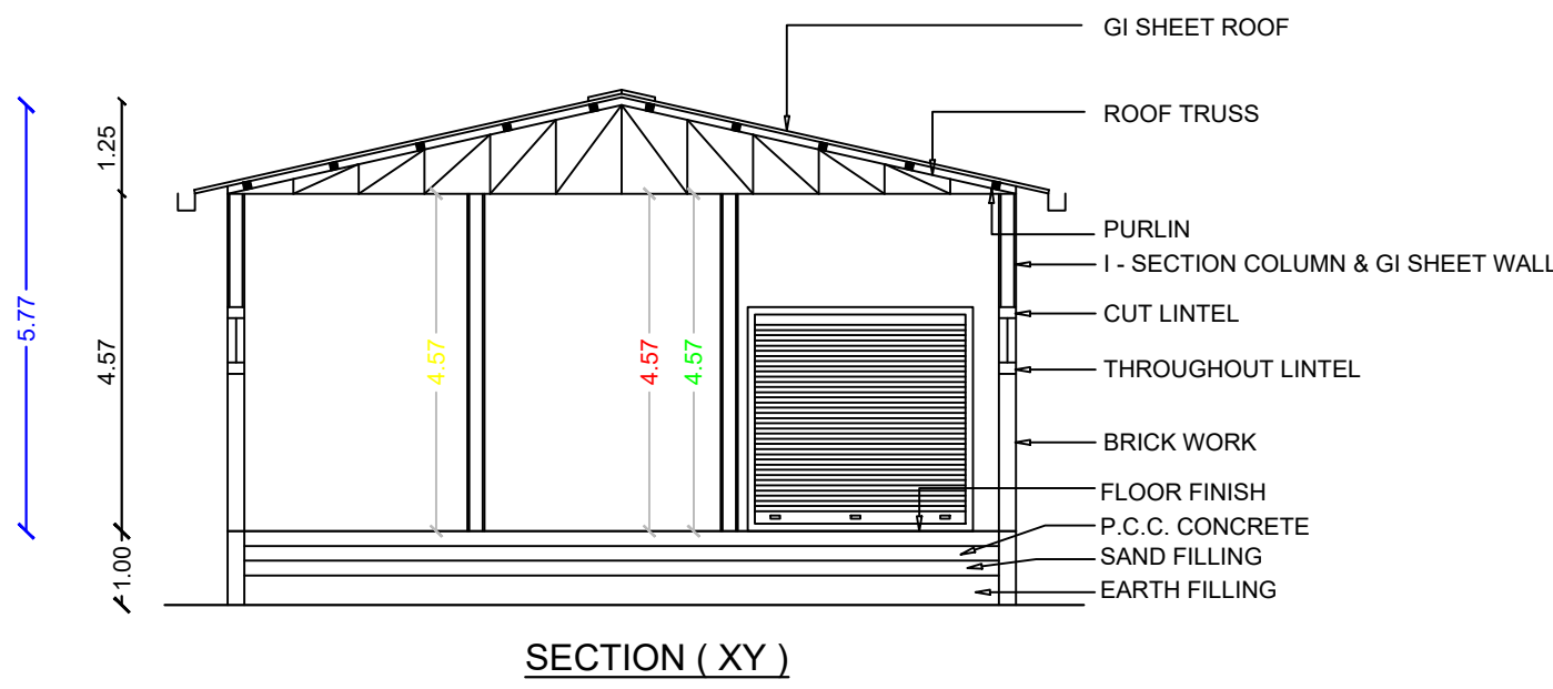
SECTION (XY)
