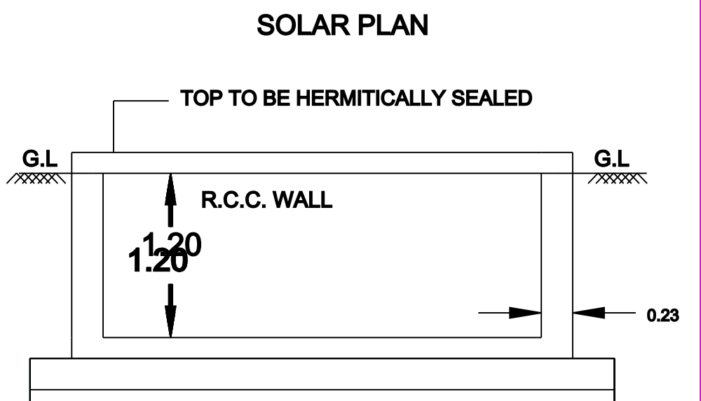
RWH SECTION
