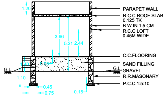
SECTION ON-AB
