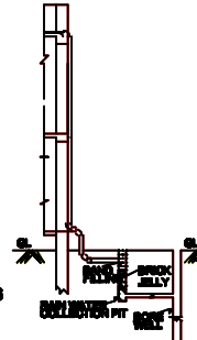
RAIN WATER HARVESTING SYSTEM 3.10M
