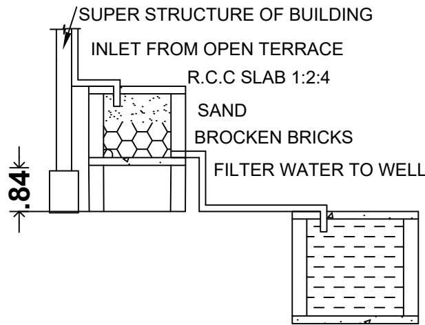
RAINWATER HARVESTING
