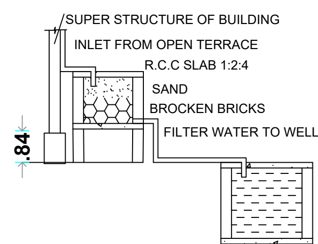
RAINWATER HARVESTING
