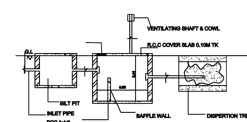
'U' TRAPS SEPTIC TANK DETAILS
