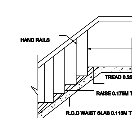
STAIRCASE DETAILS
