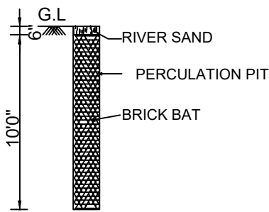
PERCOLATION PIT
