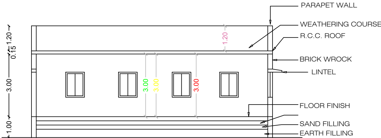
SECTION ON "XY"
