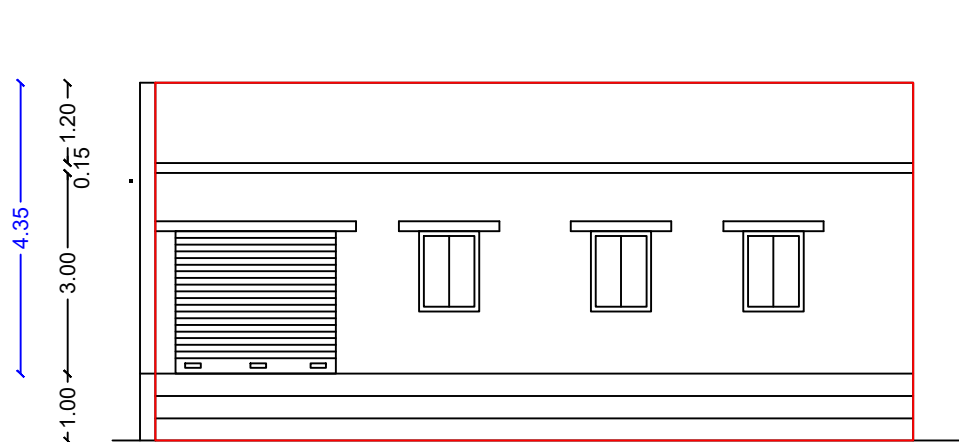
FRONT ELEVATION
