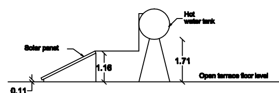
SIDE ELEVATION
