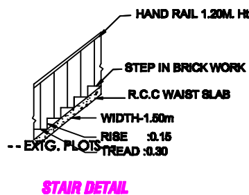
STAIR DETAIL
