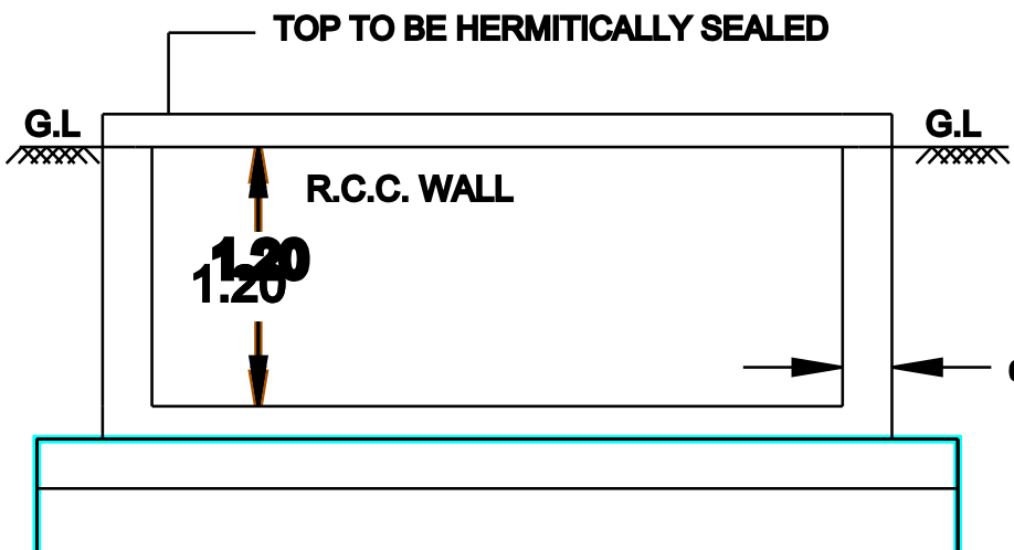
RWH SECTION
