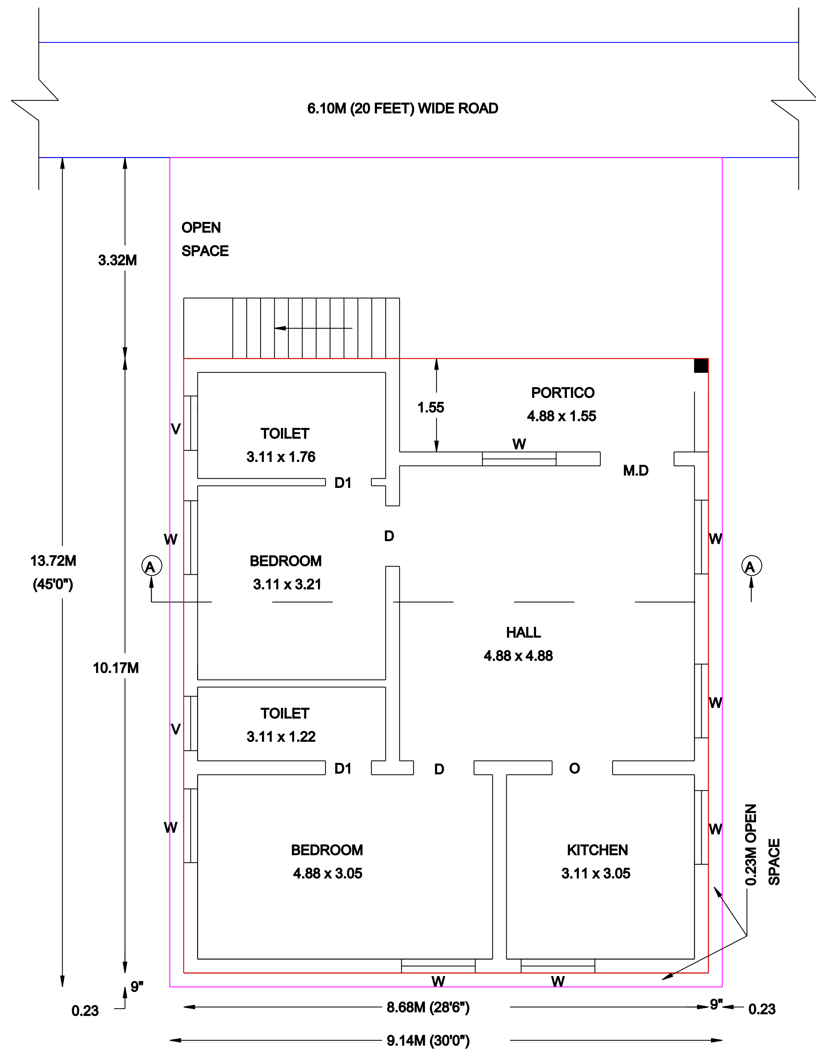
SITE CUM GROUND FLOOR PLAN
