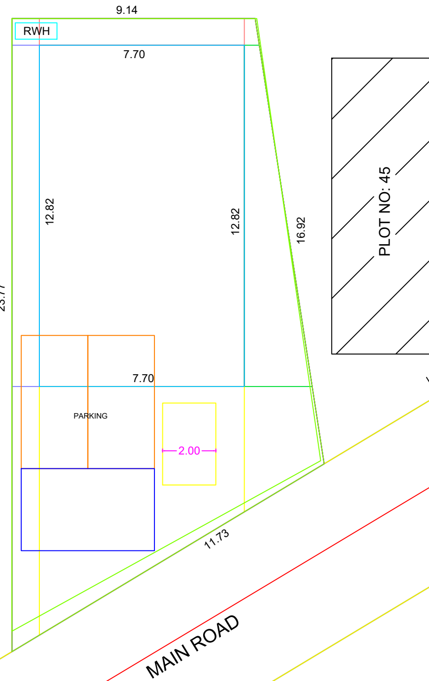
TOPO PLAN Scale 1:100
