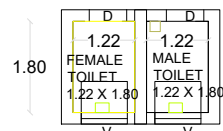
TOILET BLOCK
