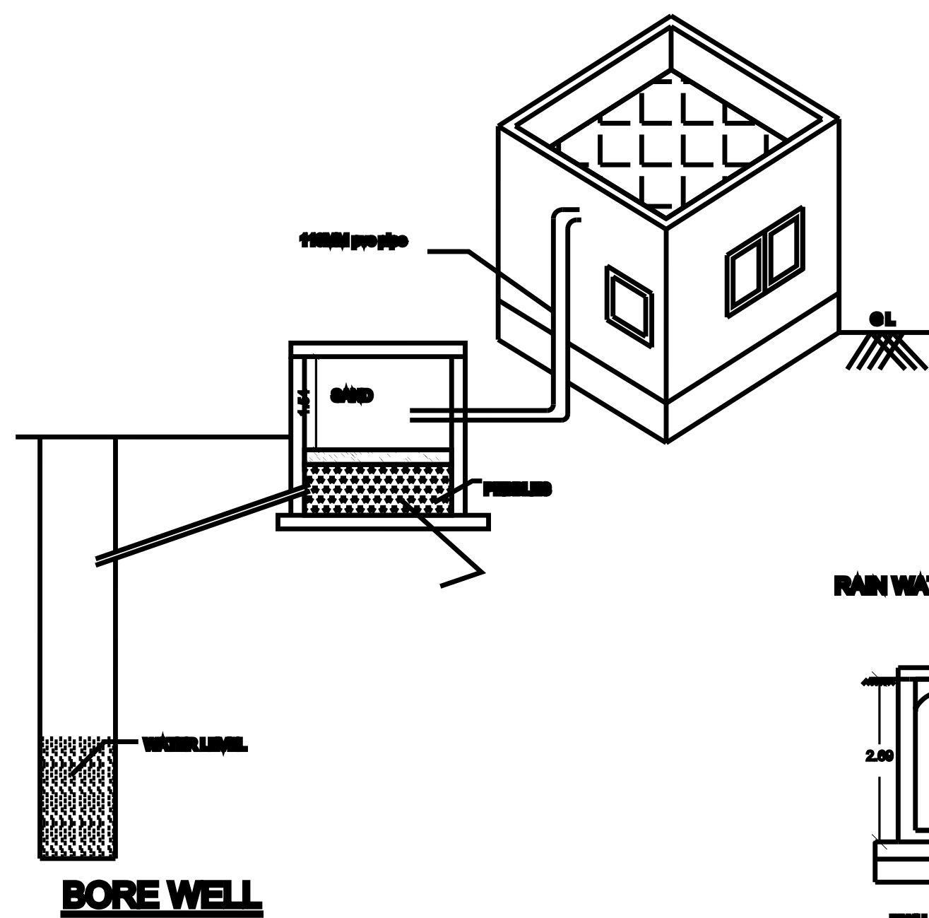
BORE WELL
