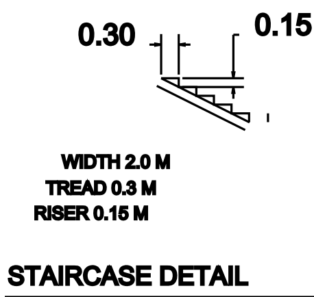
STAIRCASE DETAIL
