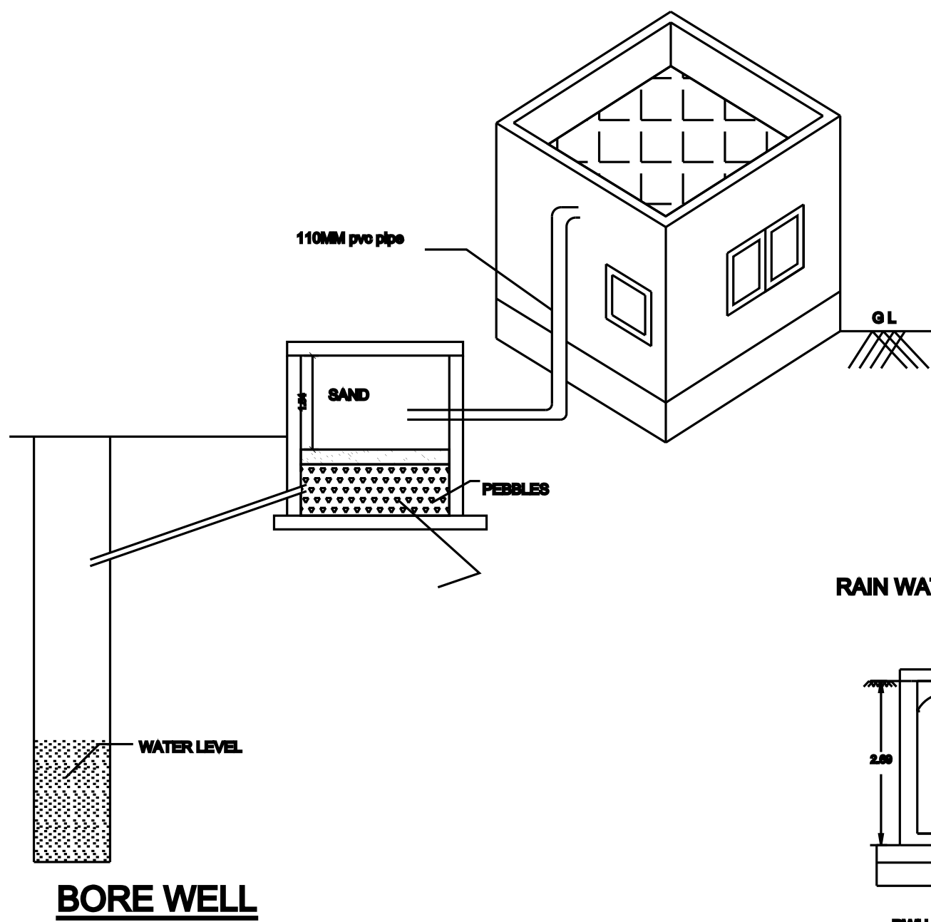
BORE WELL
