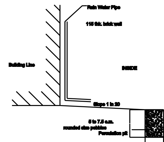
PERCOLATION PIT
