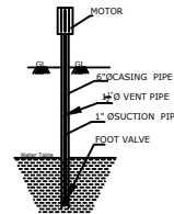
SEC. OF BOREWELL
