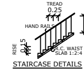
STAIRCASE DETAILS
