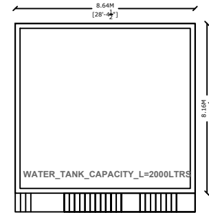
Terrace Plan
