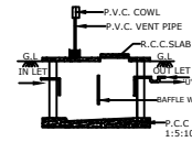
SEC. OF SEPTIC TANK
