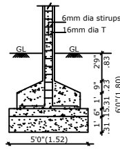
COLUMN FOUNDATION DETAIL SCALE (1:50)
