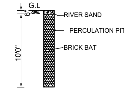
PERCOLATION PIT
