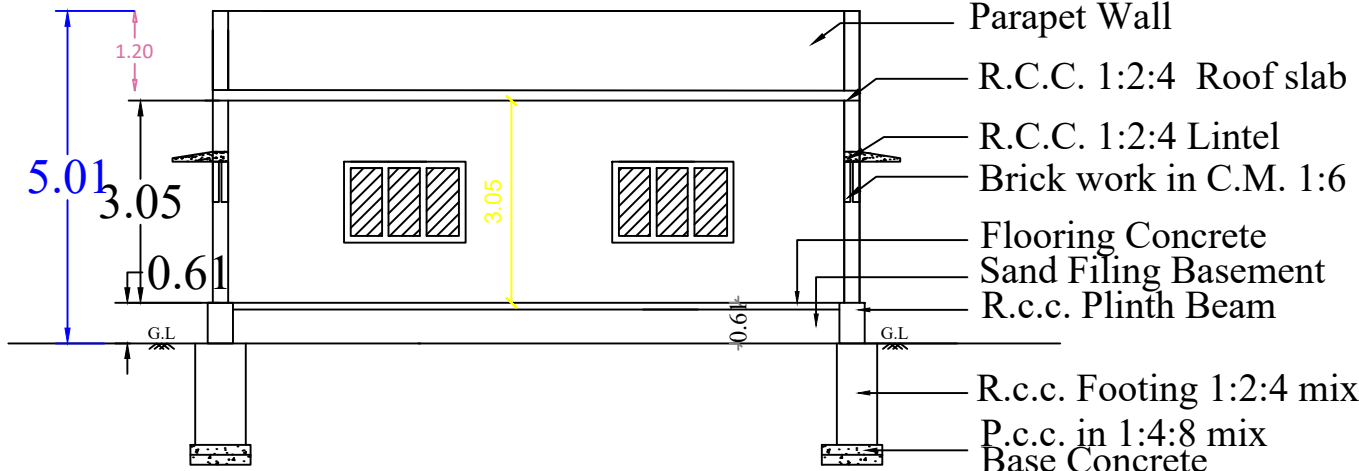
SECTION -"AB"
