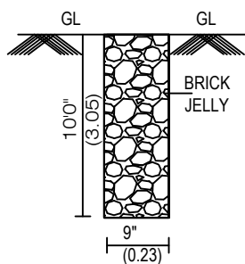
PERCOLATION PIT:-
