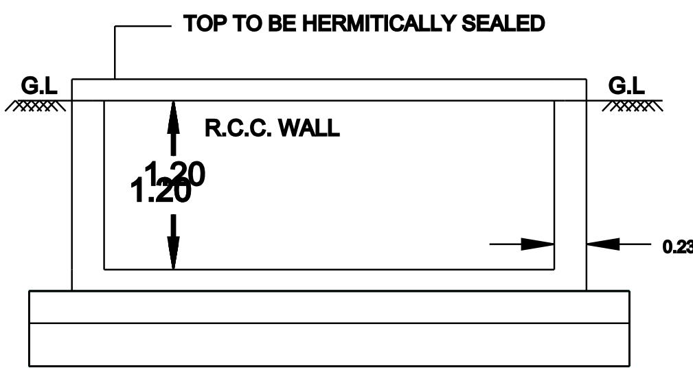
RWH SECTION
