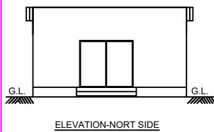
ELEVATION-NORT SIDE
