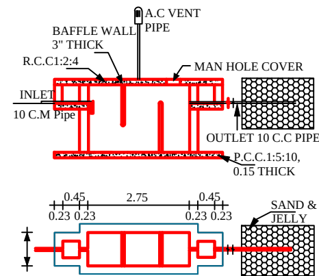
SEPTIC TANK AND TRECH
