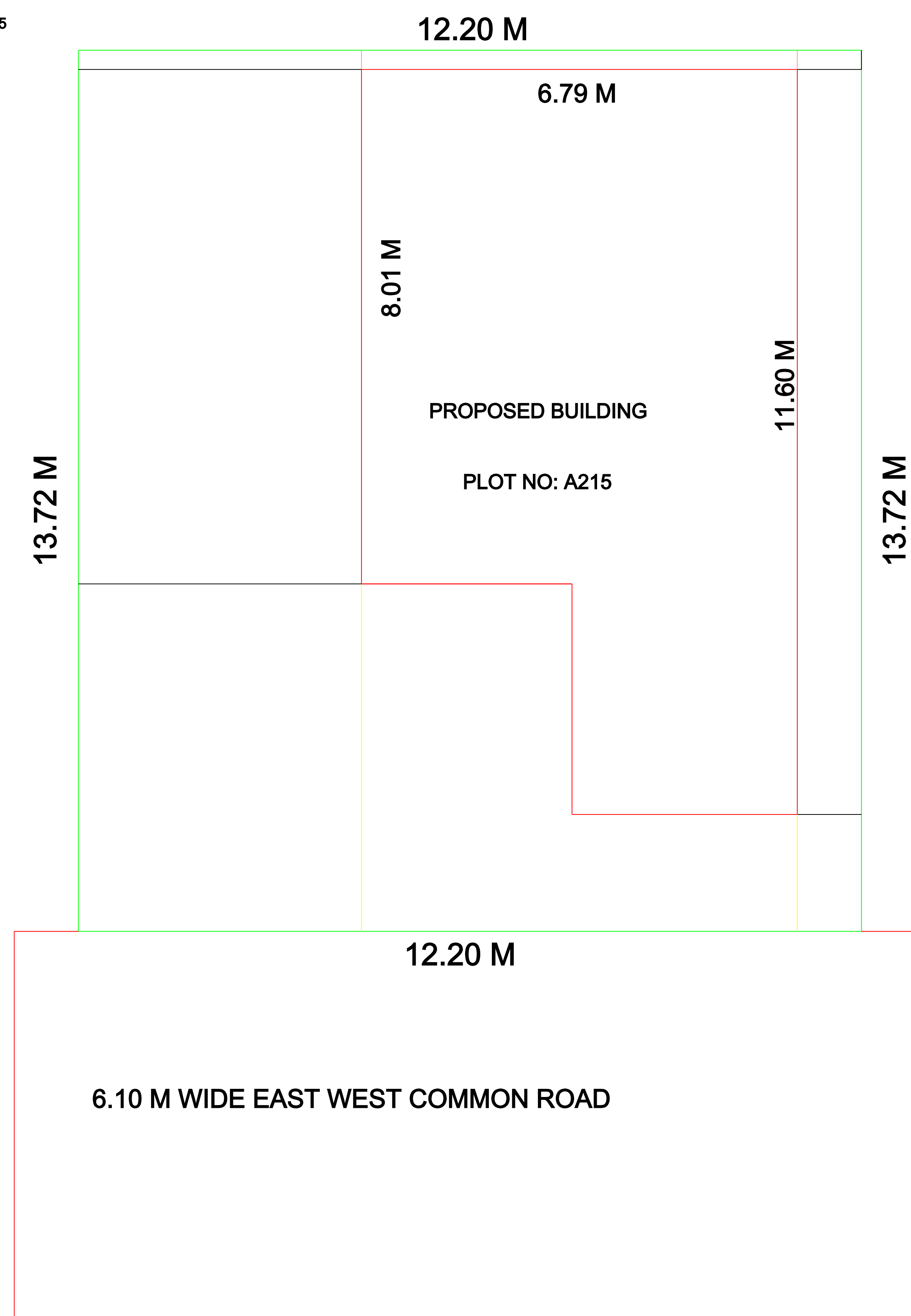
SITE PLAN
