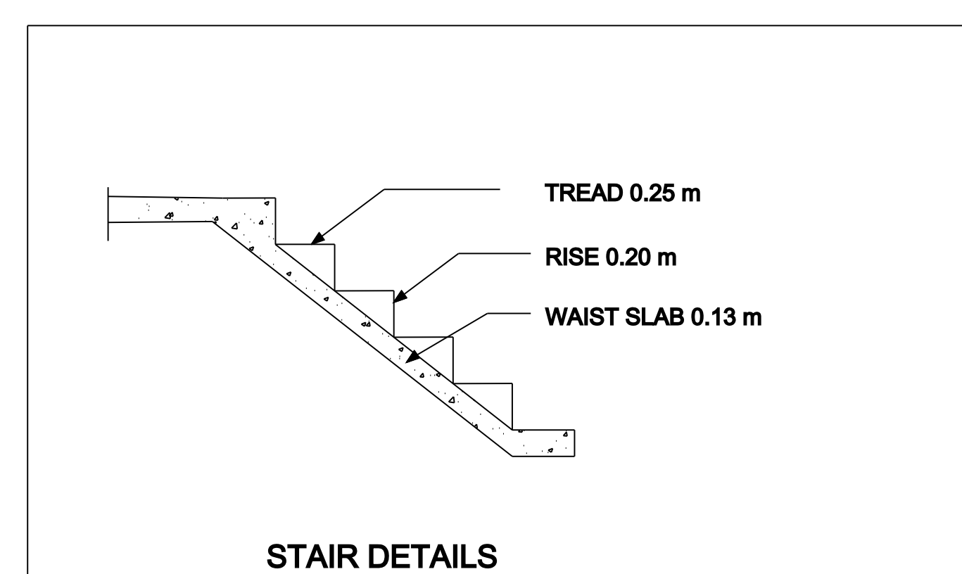
STAIR DETAILS
