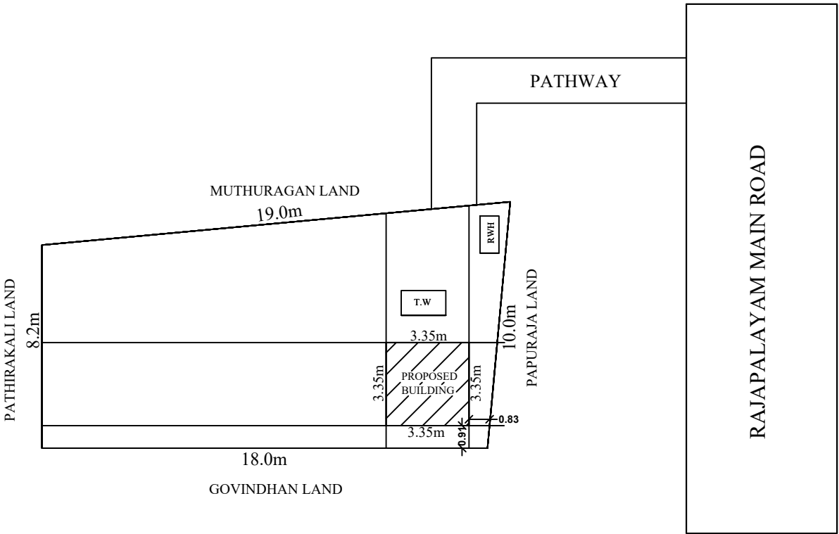
SITE PLAN
