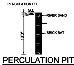
PERCOLATION PIT
