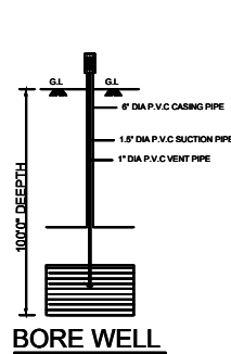
BORE WELL
