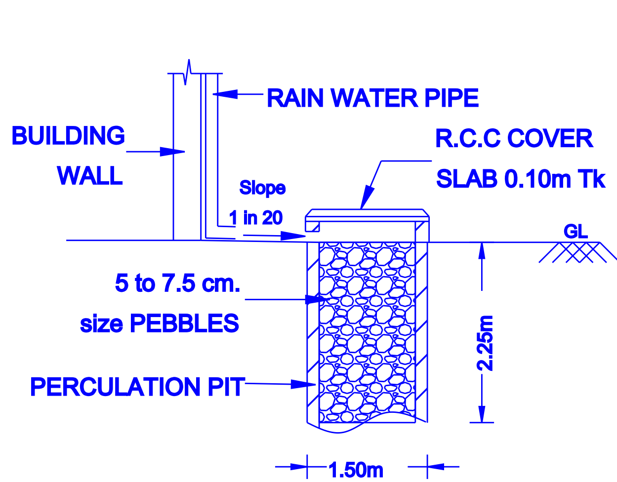
RAIN WATER HARVESTING TRENCH PIT DETAILS
