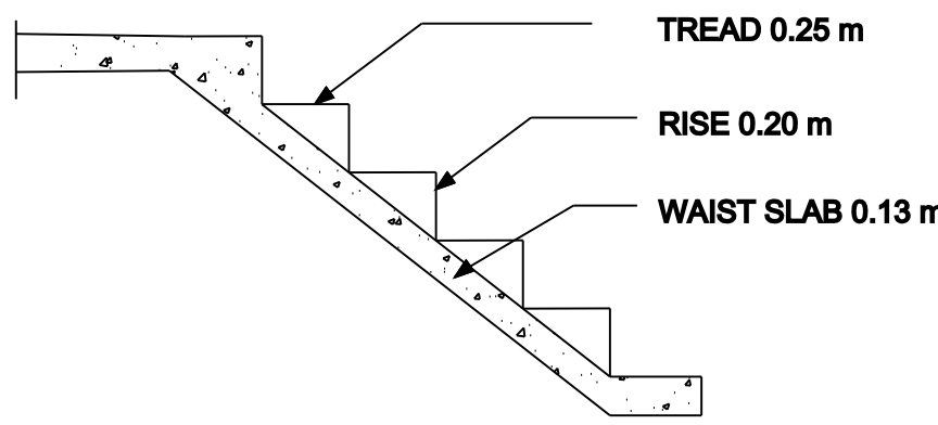
STAIR DETAILS
