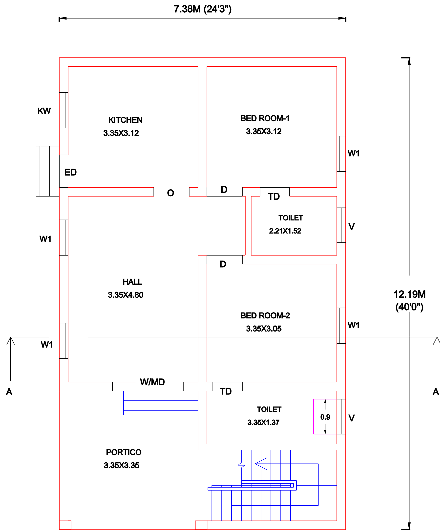
PLAN
