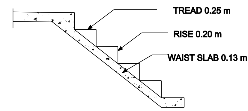
STAIR DETAILS
