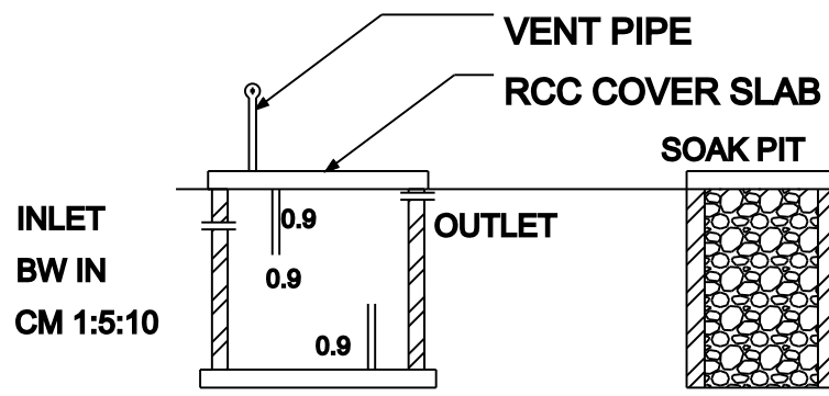
SEPTIC TANK DETAILS
