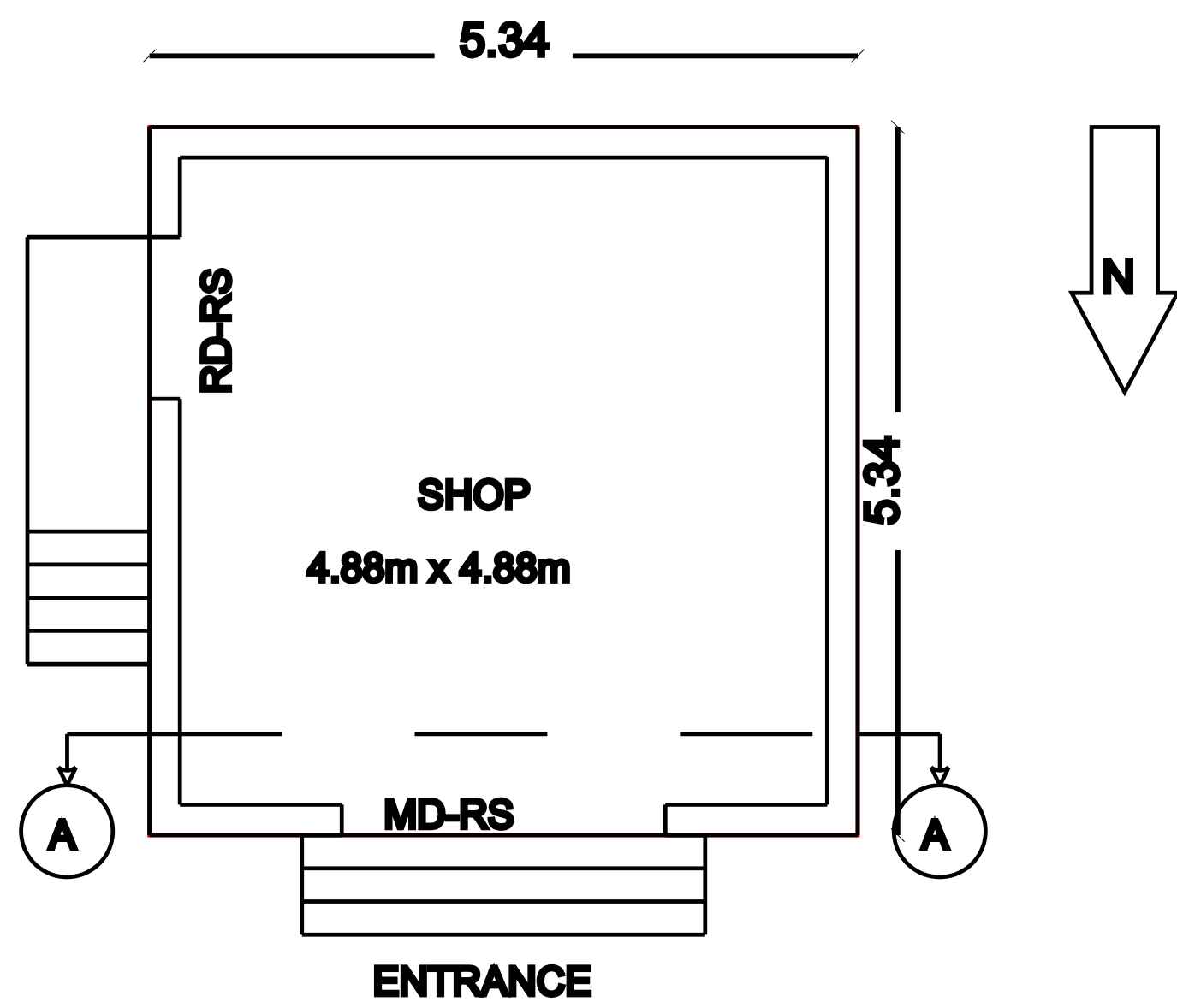
FLOOR PLAN
