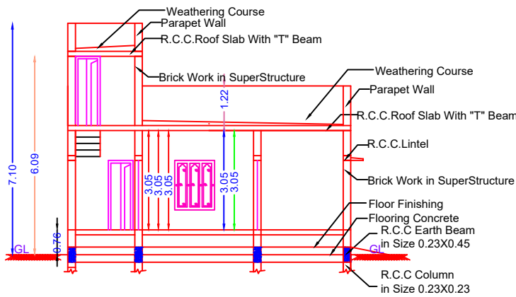
SECTION ON "PQ" (SCALE 1:100)
