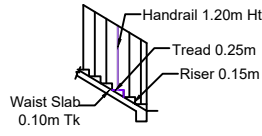
DETAILS OF STAIR CASE (SCALE 1:100)
