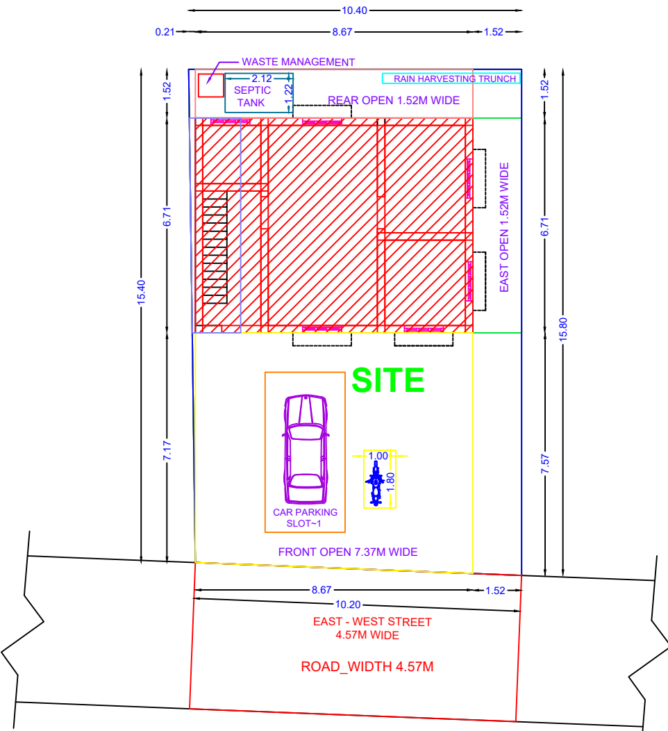
SITE PLAN
