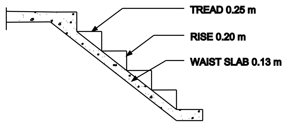
STAIR DETAILS
