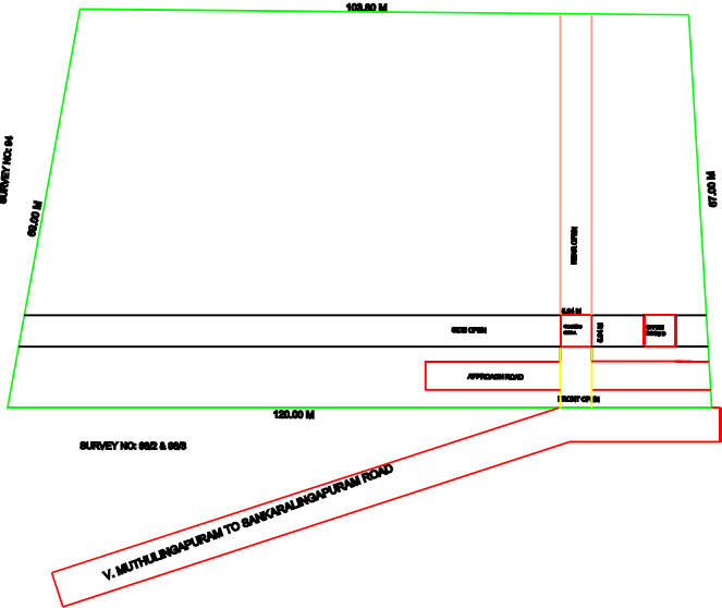
SITE PLAN
