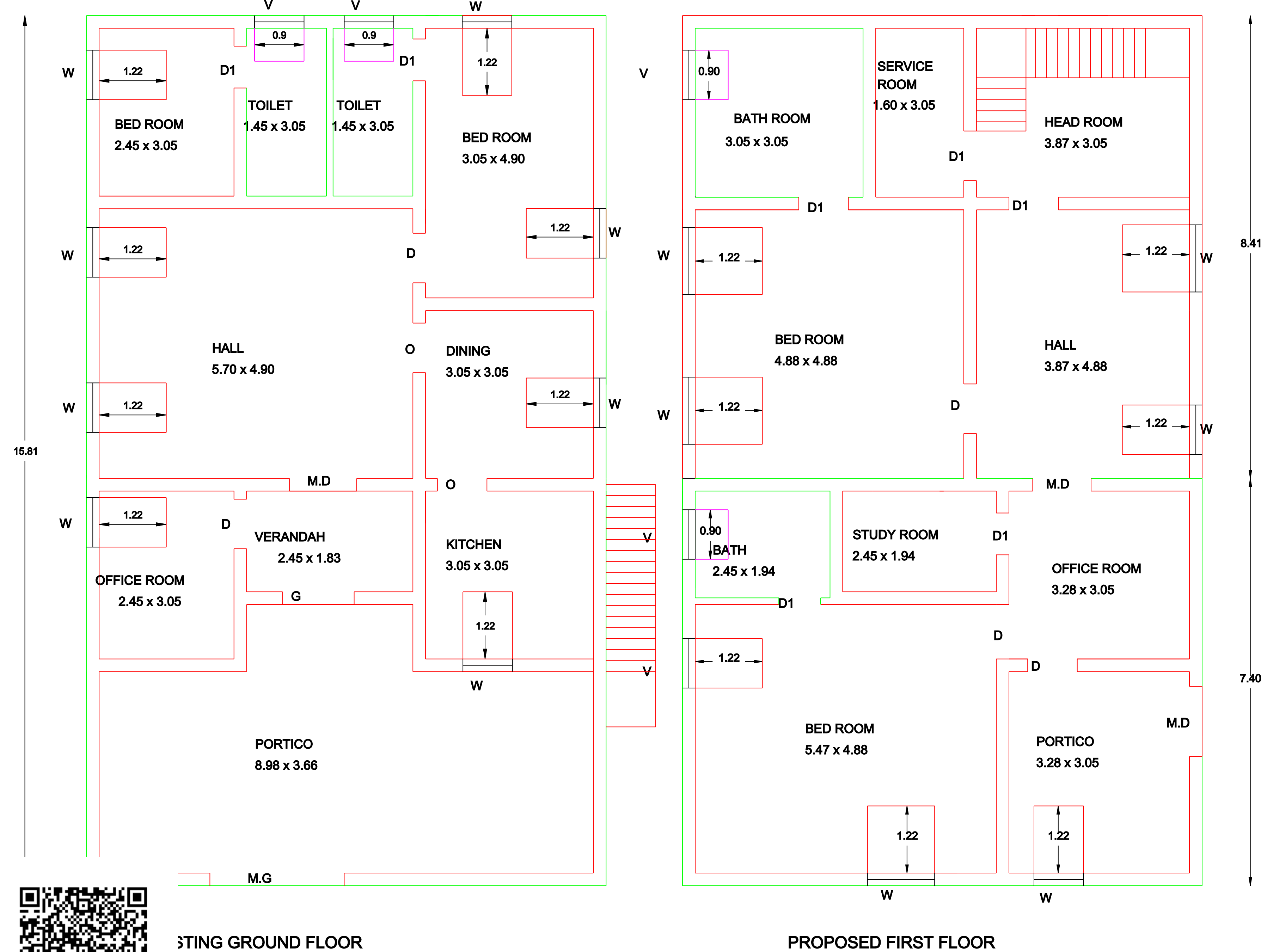
EXISTING GROUND FLOOR
