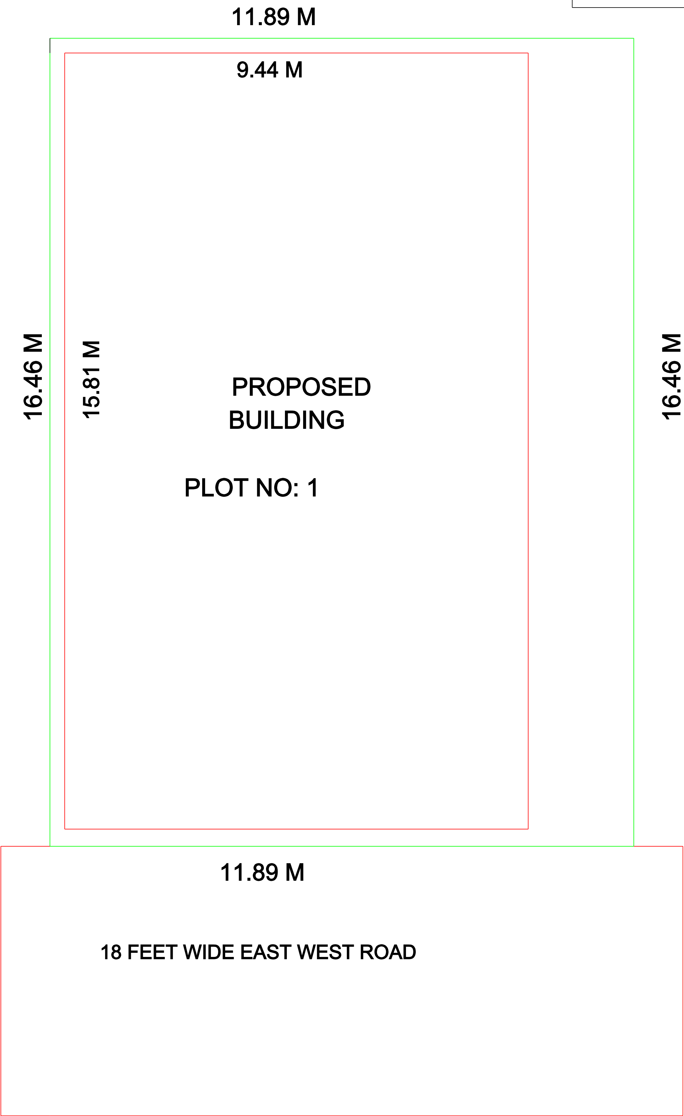
SITE PLAN
